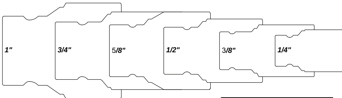
ISO 16028 Flat Face Coupler FF Series Identification Chart
